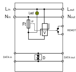
MLP2-230S-P/xx
