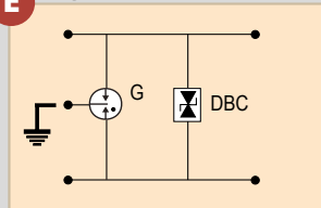
E High bit-rate Protection
