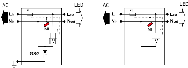
MLPM1-230L-R
