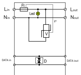
MLP2-230L-P/xx
