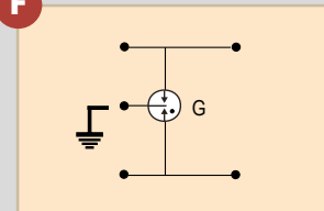
F 3-electrode GDT Protection
