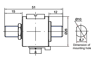
P8AX_-F/FF
