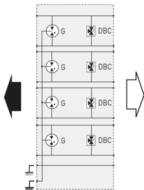
G : 3-electrode gas tube DBC : 3-pole low capacitance diode
