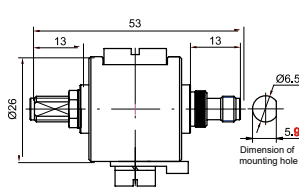
P8AX_-SMA/FF
