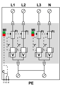
DAC15CS-40
