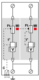
DS50PVS-500/51 DS50PVS-600/51
