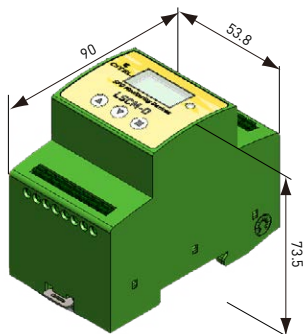
Monitoring unit LSCM-D/24
